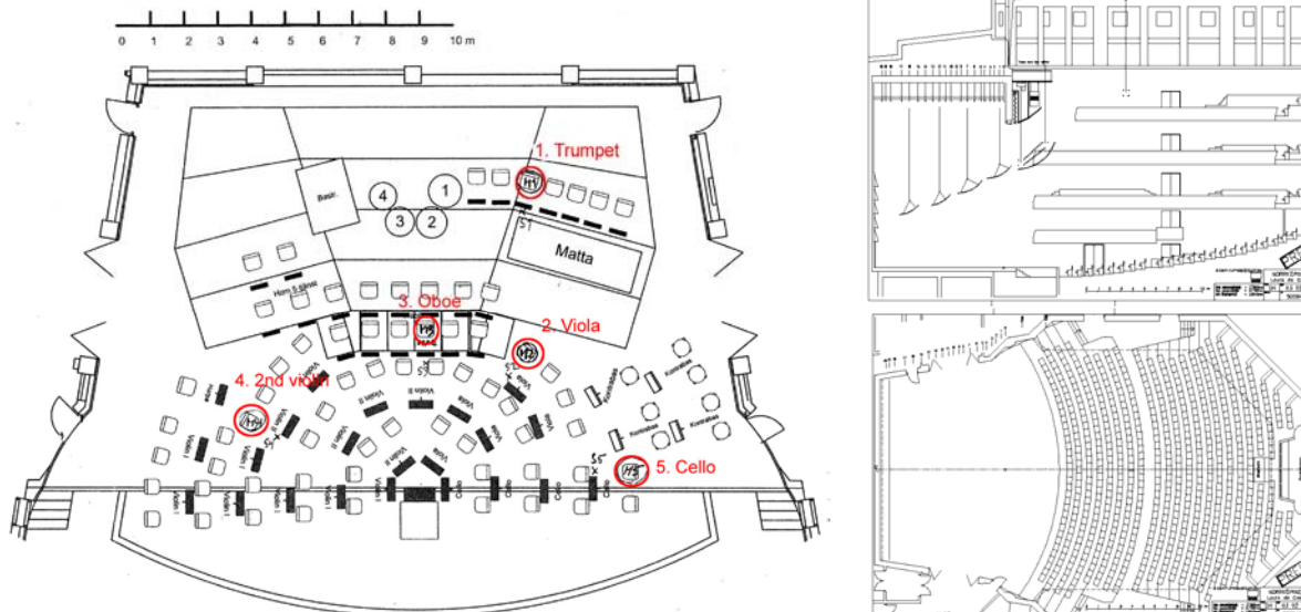
Figure 6. The De Geer hall. The five measurement positions on stage in the original placement of the orchestra (left). Cross section and plan (right). Note that the heights of the ceiling reflectors are not the one used.
