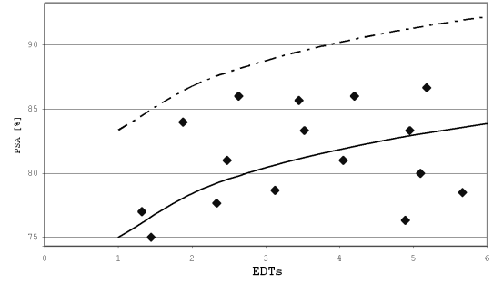
Fig. 10. EDT_s coefficient against corresponding, averaged PSA in 16 measurement points for condition with disturbing noise. Dotted line presents tendency obtained without background noise, solid line shows estimated tendency with background noise. Solid line was drawn using equation y = 4.95 \ln(EDT_s) + 75 comparing to the dotted line using equation y = 4.95 \ln(EDT_s) + 83.335 .
