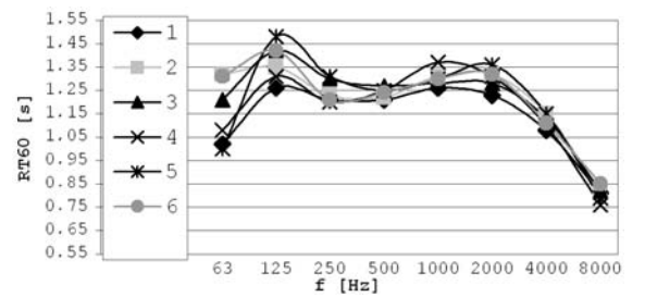
Fig. 7. RT60 curves for 6 measurement points. Points indicated with gray background and indicators p1, p2, p3, p4, p5 and p6 on the Fig. 4.
