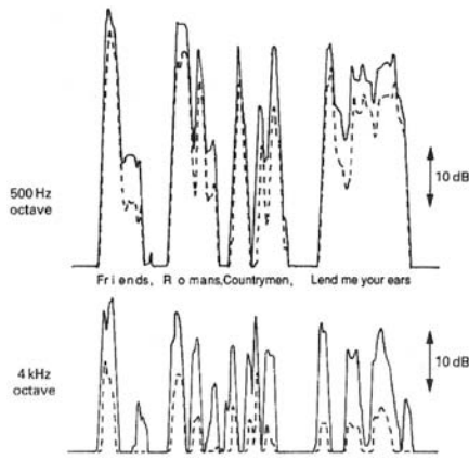
Fig. 2. Sound level vs. time for speech phrase at low mid and high frequencies. Solid line — in front of the speaker, dotted line — behind speaker [5].
