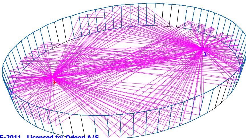
Odeon©1985-2011 Licensed to: Odeon A/S Figure 7. Elliptical room with dimensions (l \times b \times h) = (30, 20, 4) metres. All surfaces are smooth with just 1% scattering. Ceiling and floor are 80% absorbing and walls consists of concrete. Direct sound path , first and second order reflections are displayed.
